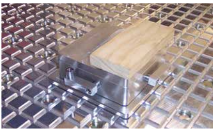
Vacuum ON, locator pins "down"
