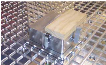
Vacuum OFF, locator pins "up"
